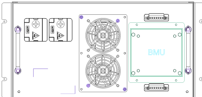
Fig.6 Silkscreen Diagram
