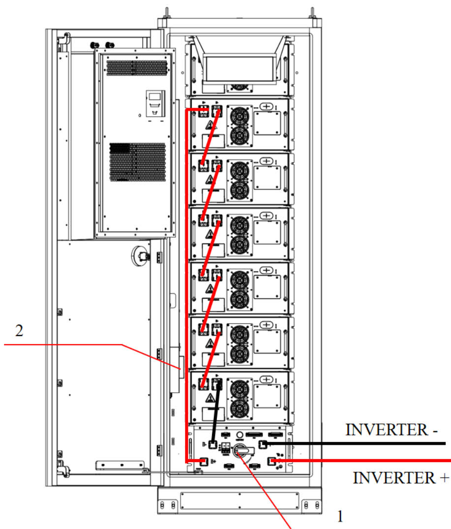
Fig.14 Operation Switch Position Diagram
