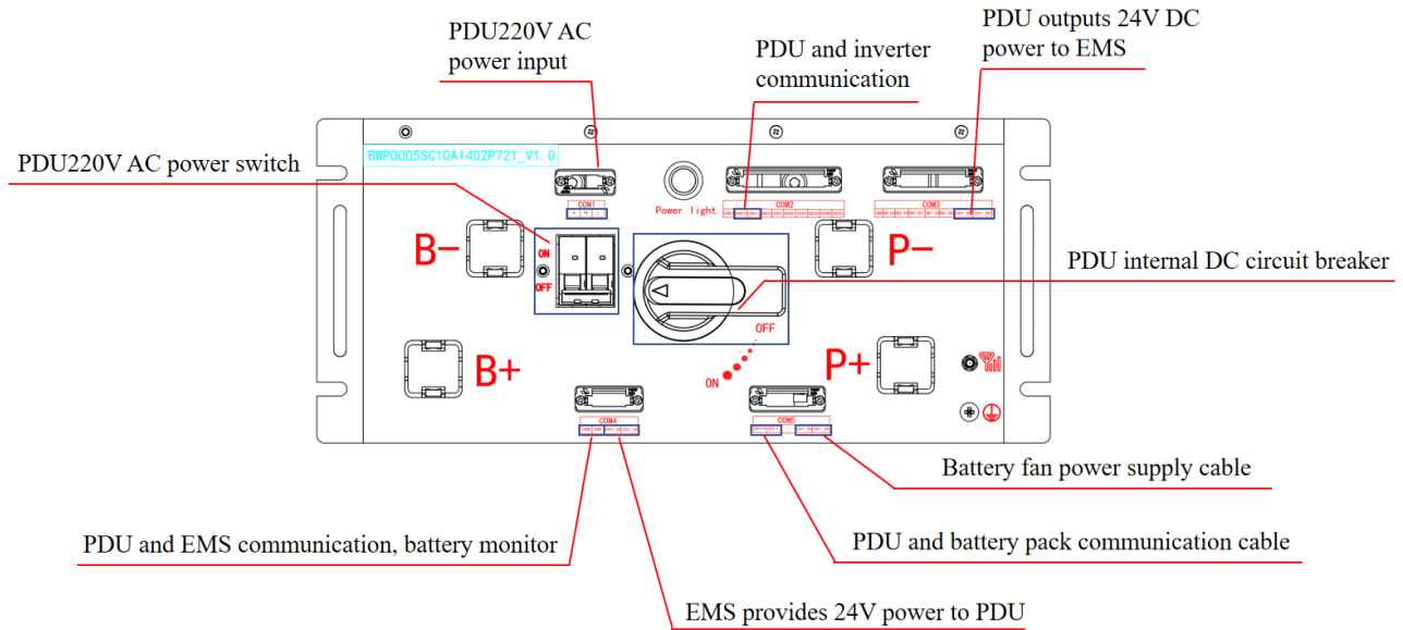
Fig.8 Silkscreen Diagram
