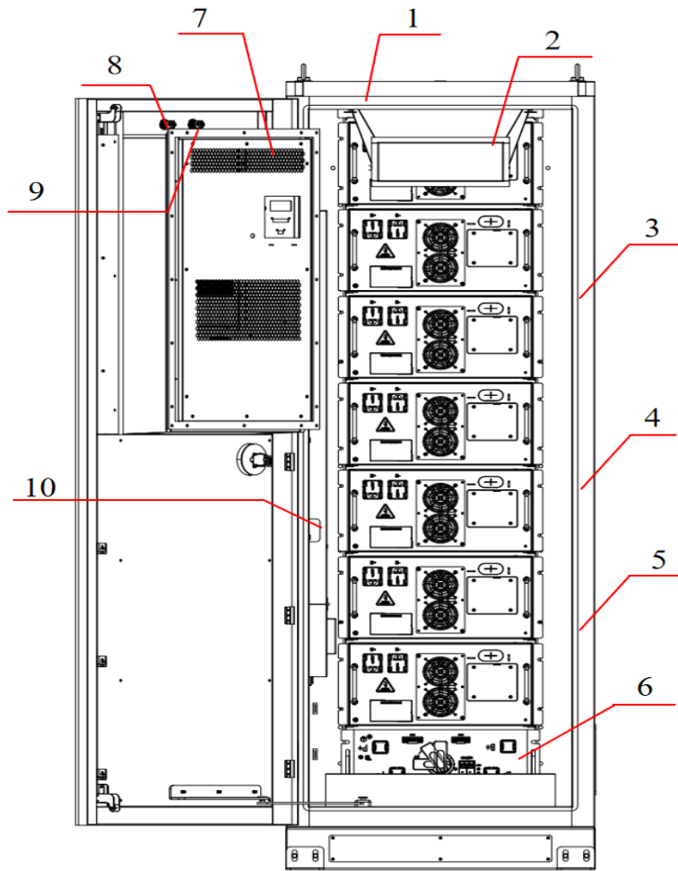
Fig.4 Main Equipment
