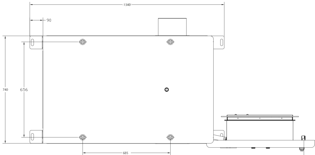
Fig.10 Reference Drawing of the Base Installation Size
