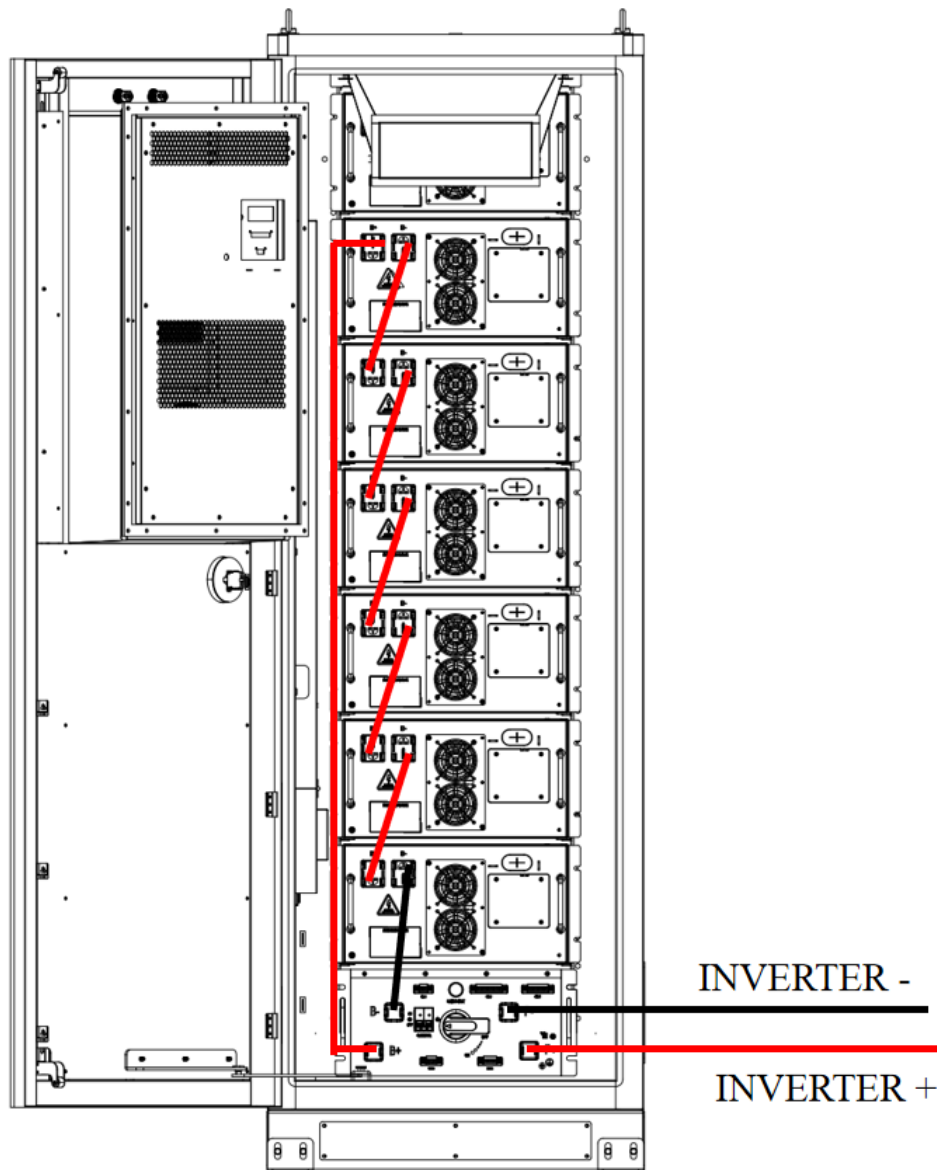
Fig.12 Power, Communication Line Connection Diagram Between Battery Box
