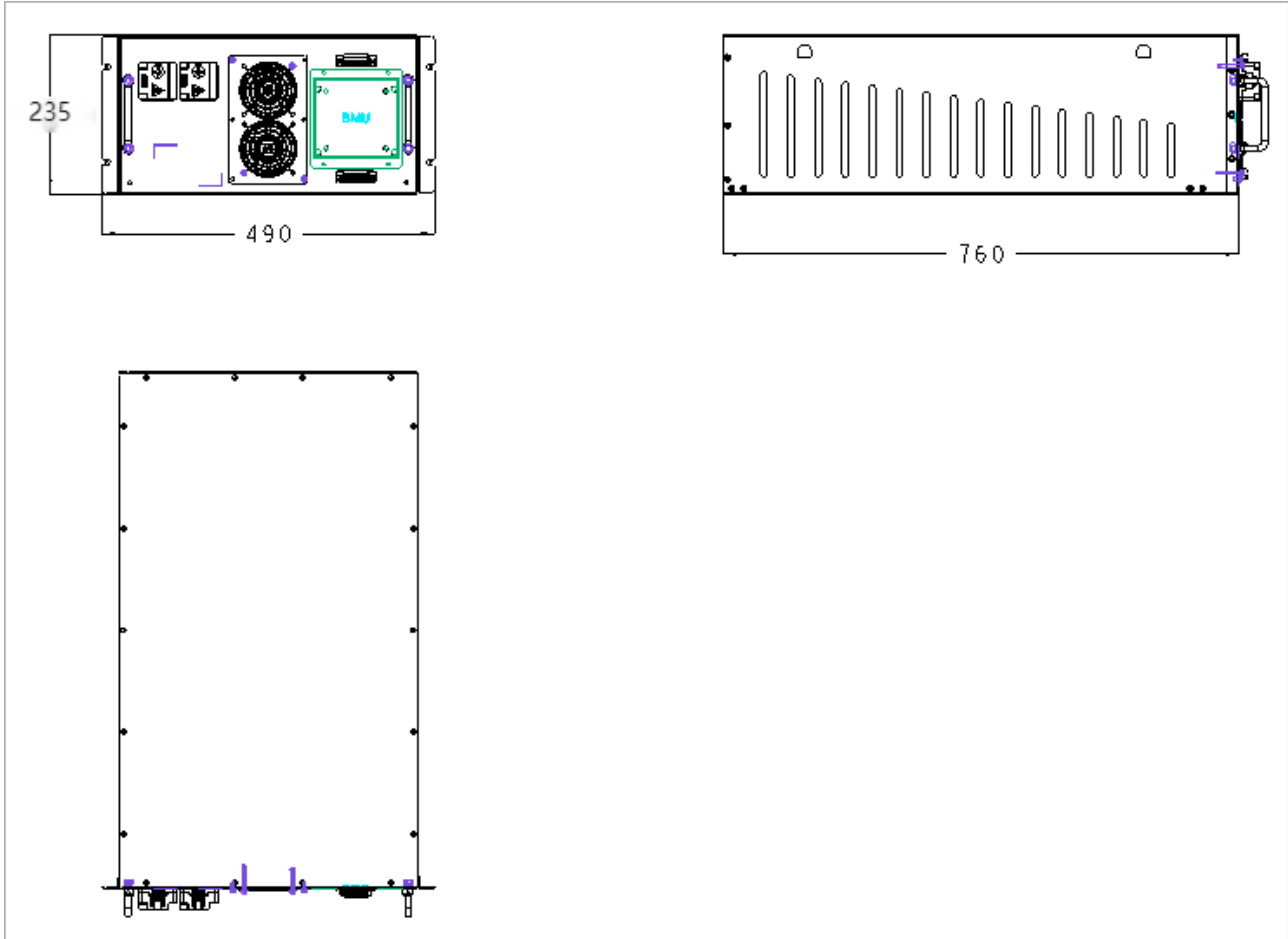
Fig.5 LCS Battery Box Dimension
