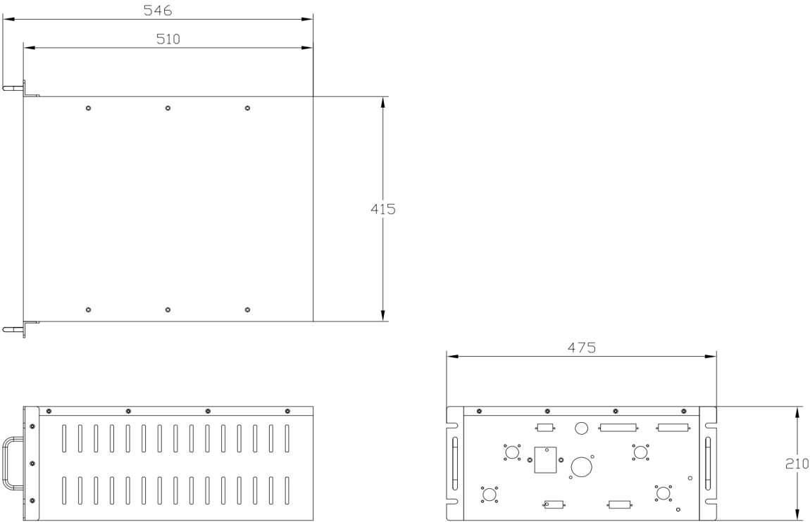
Fig.7 Overall Dimension
