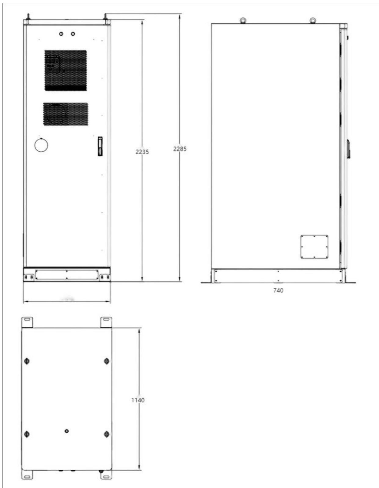
Fig.3 Overall Dimensions
