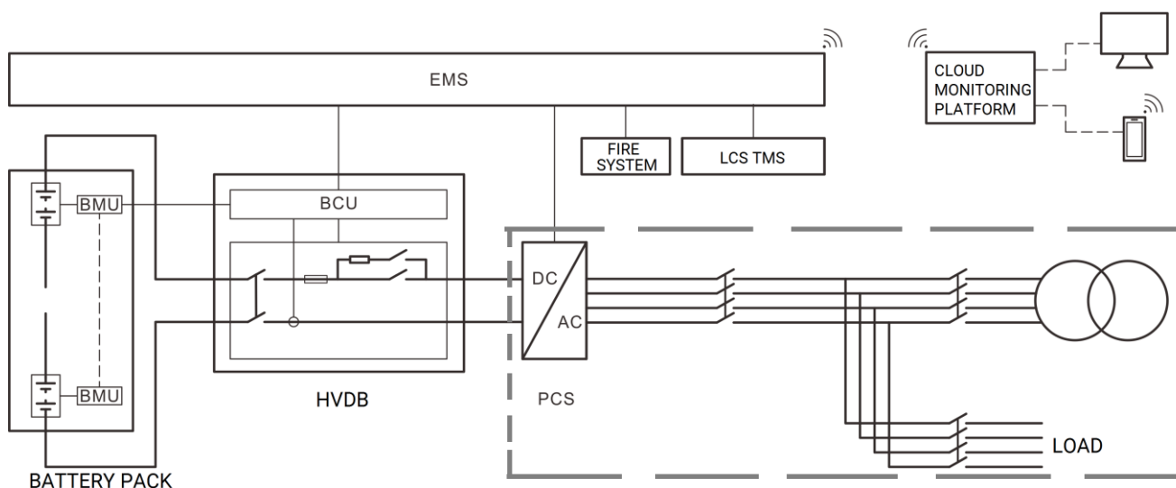
Fig.1 Topology Diagram
