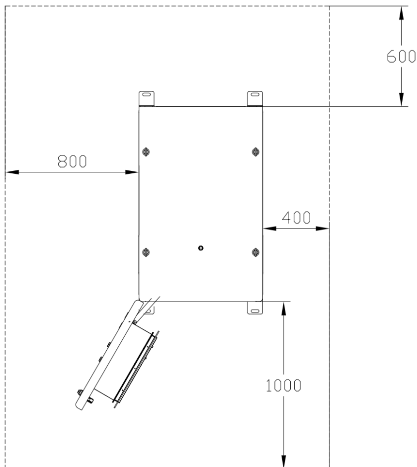
Fig.11 Reference Drawing of Installation Space Size
